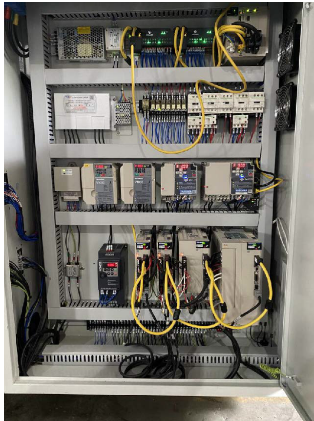
Electrical Components
