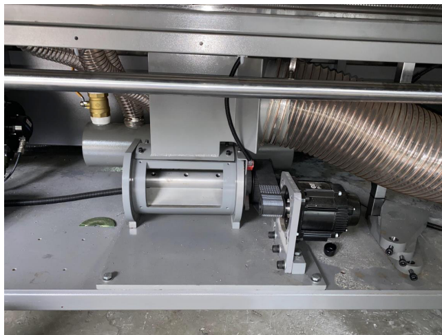
Bottom Suction and Feeding Servo Motor
