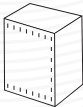
Bottom stitching of full flap slotted container.
