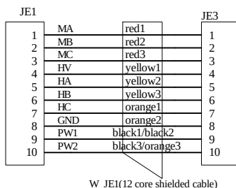
W_JE1(12 core shielded cable)
