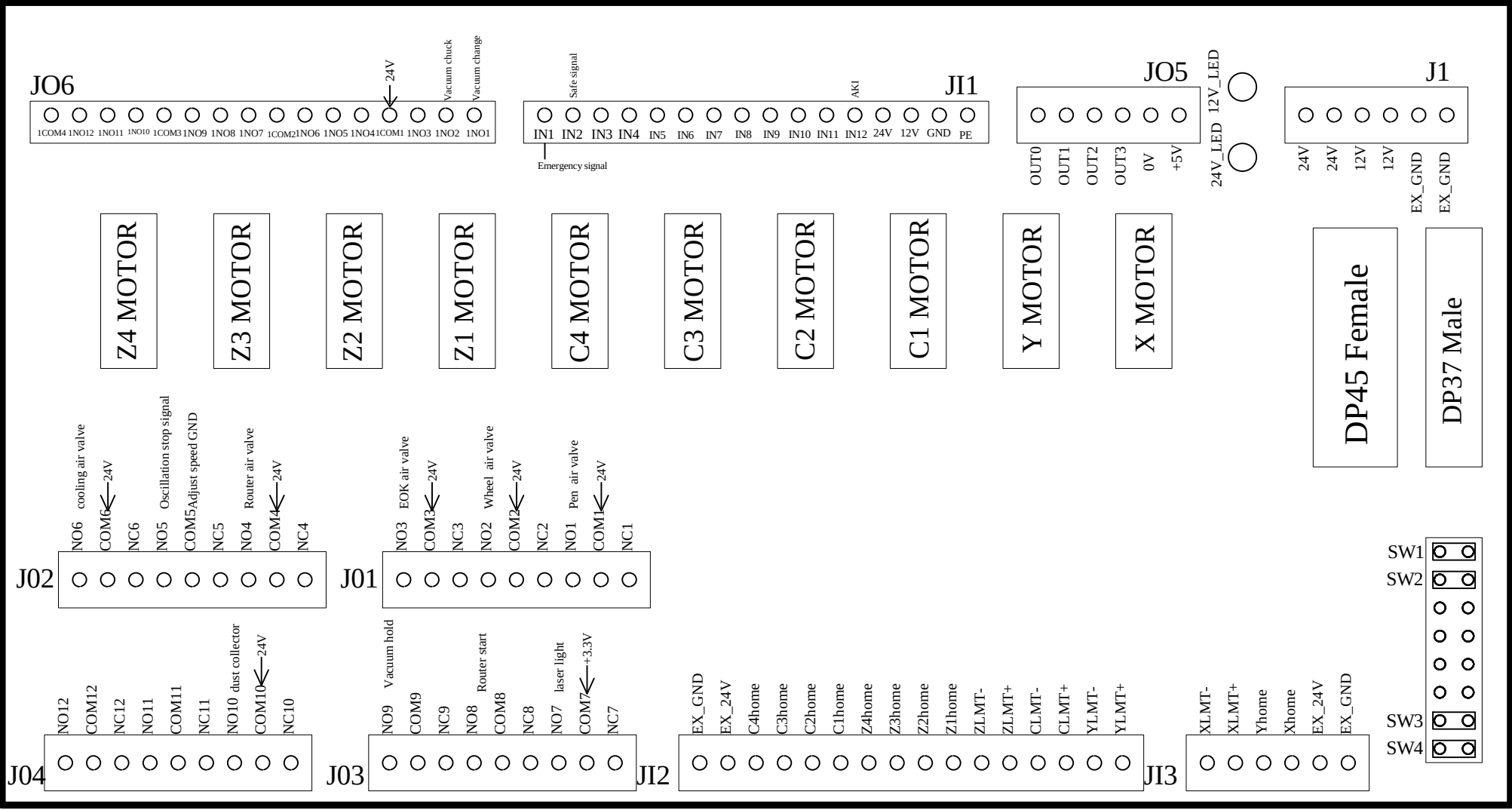
DCZ75 Interface board
